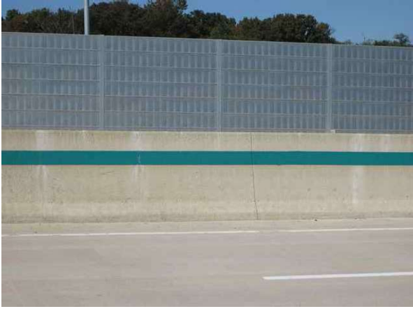
S3 방호벽 균열(0.2mm/1.5m)
