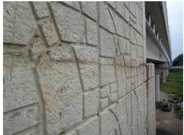
A2 균열 (0.2mm/3.0m)
