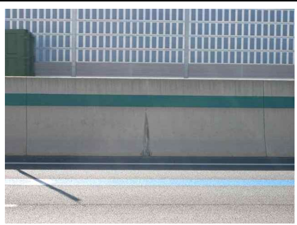
S5 균열 (0.2mm/1.5m)
